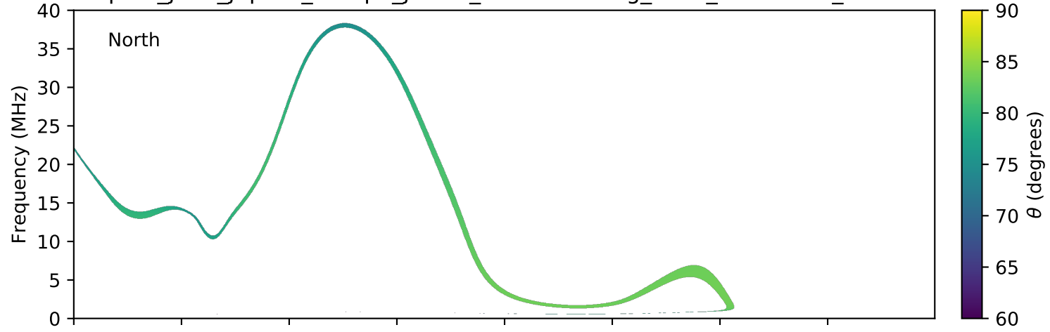
expres_juno_jupiter_europa_jrm09_lossc-wid1deg_3kev_20180308_v01.cdf
