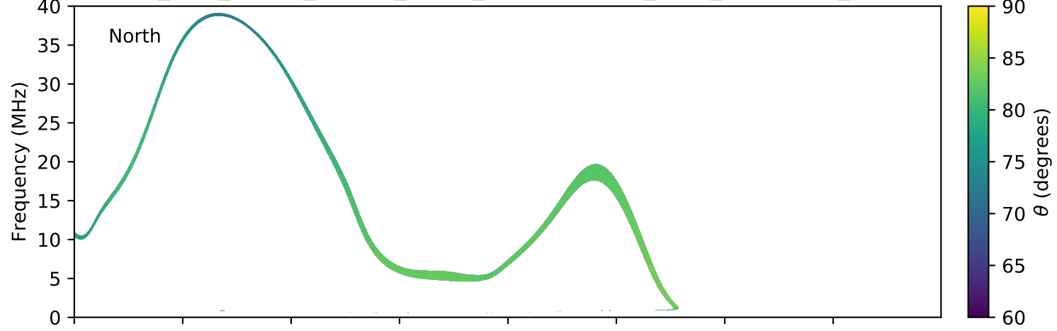
expres_juno_jupiter_europa_jrm09_lossc-wid1deg_3kev_20180304_v01.cdf
