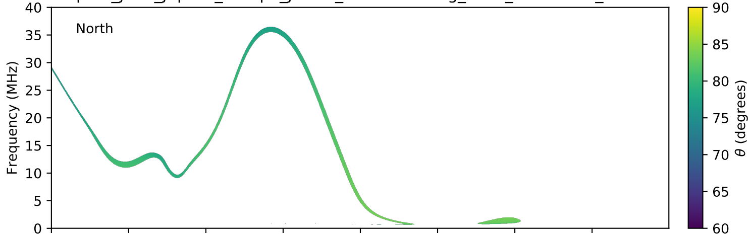
expres_juno_jupiter_europa_jrm09_lossc-wid1deg_3kev_20180303_v01.cdf
