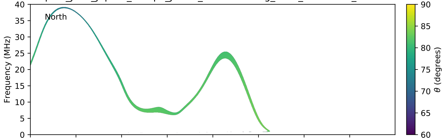
expres_juno_jupiter_europa_jrm09_lossc-wid1deg_3kev_20180302_v01.cdf
