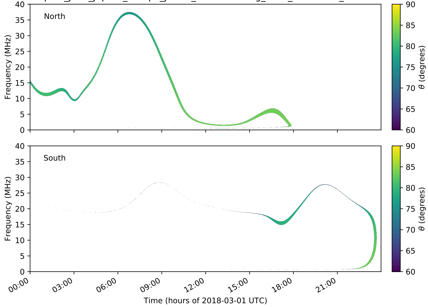
expres_juno_jupiter_europa_jrm09_lossc-wid1deg_3kev_20180301_v01.cdf
