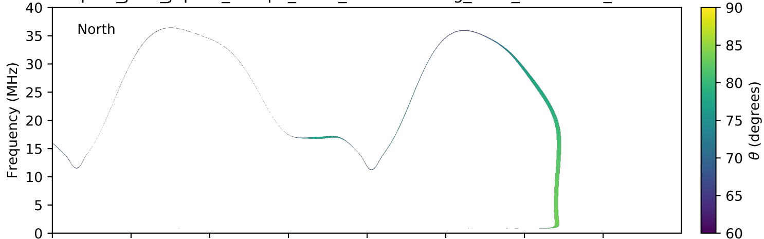
expres_juno_jupiter_europa_isaac_lossc-wid1deg_3kev_20180330_v01.cdf
