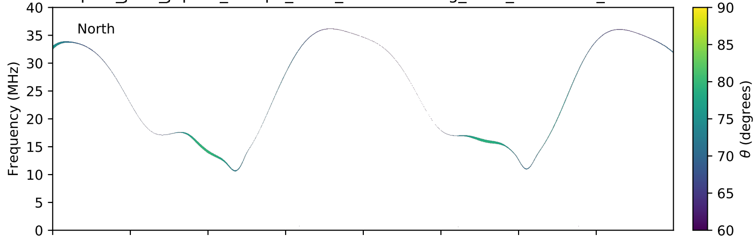
expres_juno_jupiter_europa_isaac_lossc-wid1deg_3kev_20180326_v01.cdf
