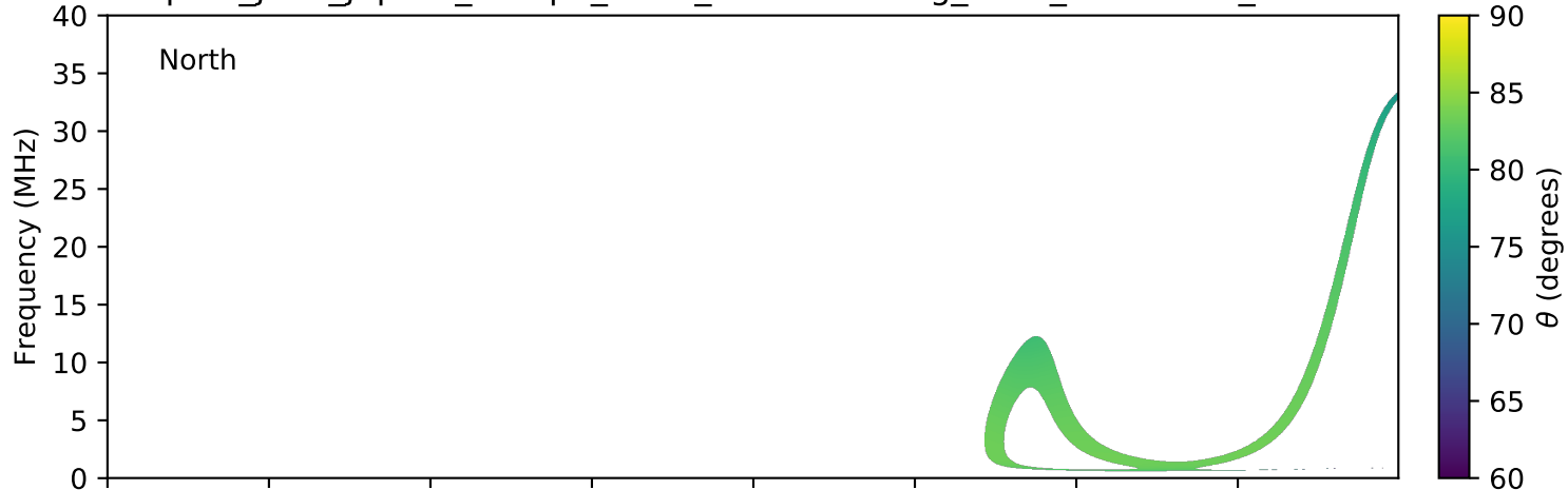
expres_juno_jupiter_europa_isaac_lossc-wid1deg_3kev_20180325_v01.cdf
