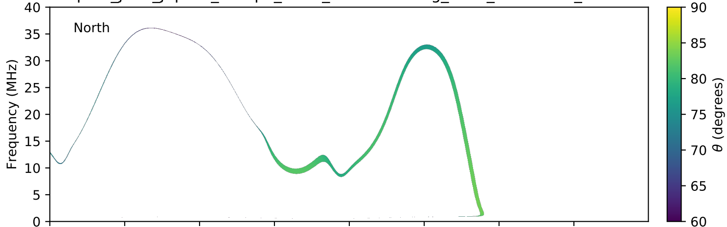
expres_juno_jupiter_europa_isaac_lossc-wid1deg_3kev_20180323_v01.cdf
