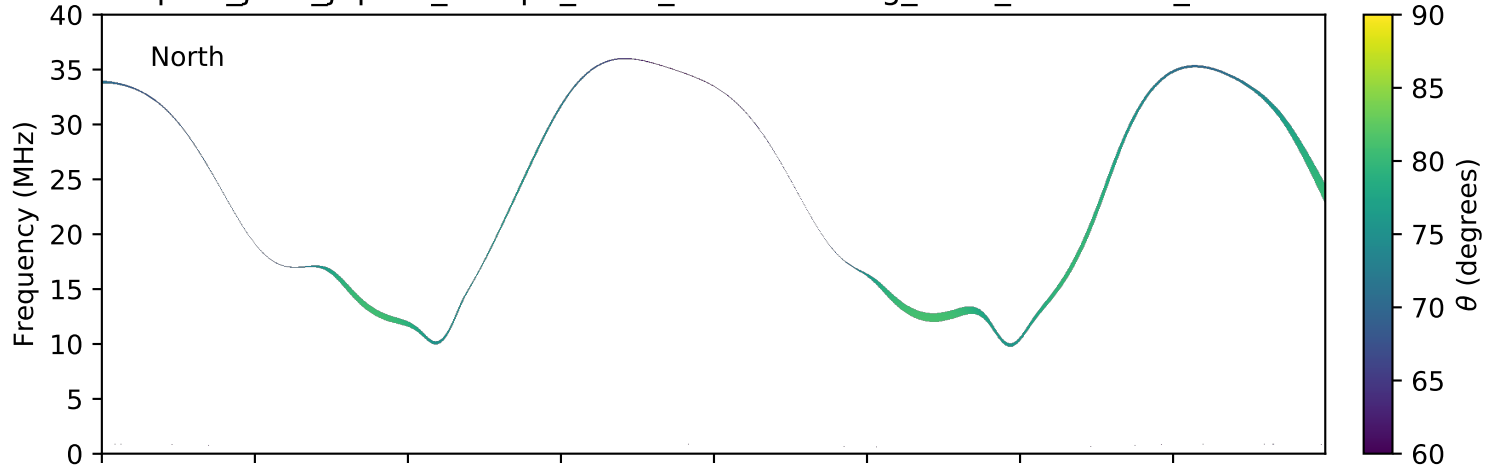
expres_juno_jupiter_europa_isaac_lossc-wid1deg_3kev_20180319_v01.cdf
