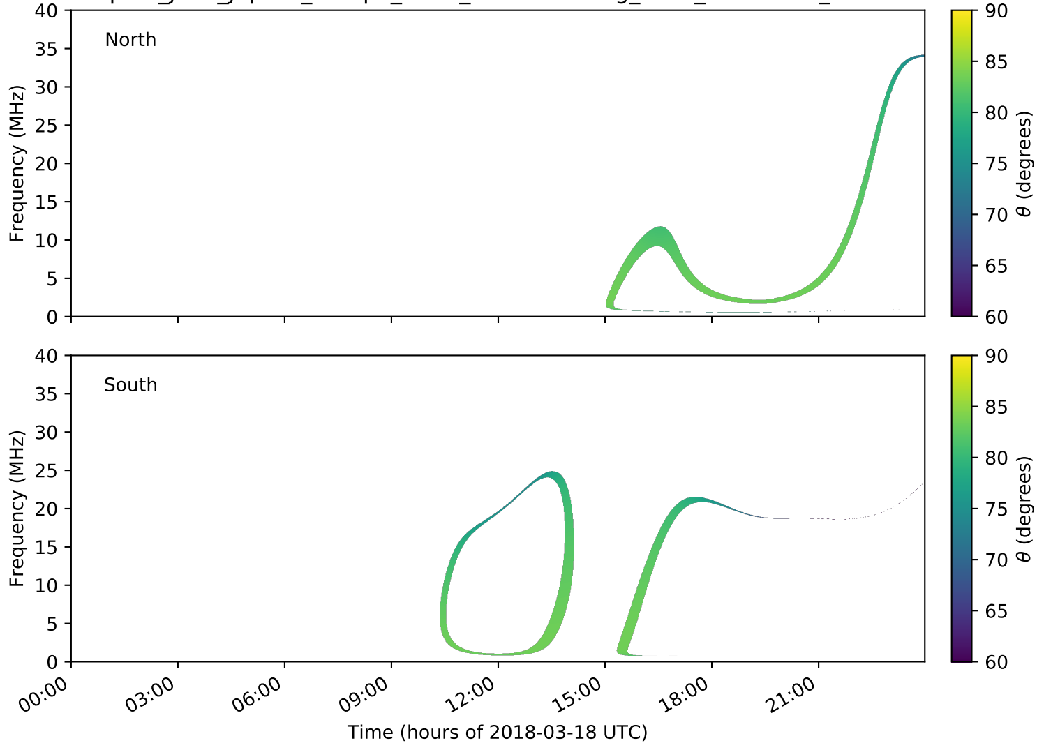
expres_juno_jupiter_europa_isaac_lossc-wid1deg_3kev_20180318_v01.cdf
