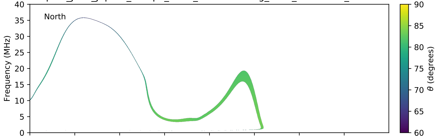
expres_juno_jupiter_europa_isaac_lossc-wid1deg_3kev_20180316_v01.cdf
