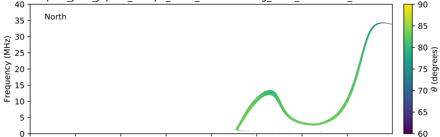
expres_juno_jupiter_europa_isaac_lossc-wid1deg_3kev_20180311_v01.cdf
