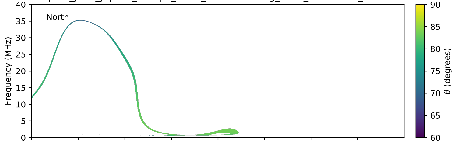
expres_juno_jupiter_europa_isaac_lossc-wid1deg_3kev_20180309_v01.cdf
