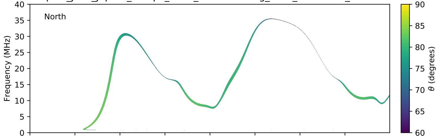
expres_juno_jupiter_europa_isaac_lossc-wid1deg_3kev_20180308_v01.cdf
