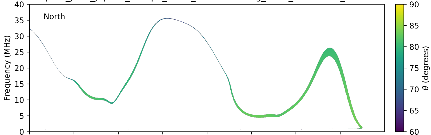
expres_juno_jupiter_europa_isaac_lossc-wid1deg_3kev_20180305_v01.cdf
