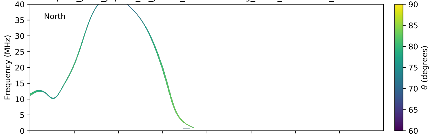
expres_juno_jupiter_io_jrm09_lossc-wid1deg_3kev_20180222_v01.cdf
