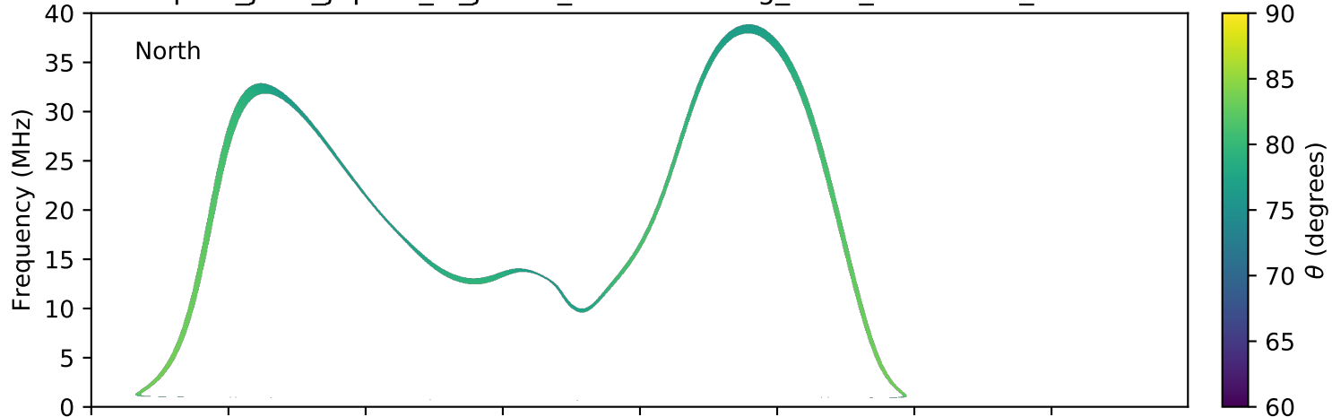
expres_juno_jupiter_io_jrm09_lossc-wid1deg_3kev_20180220_v01.cdf
