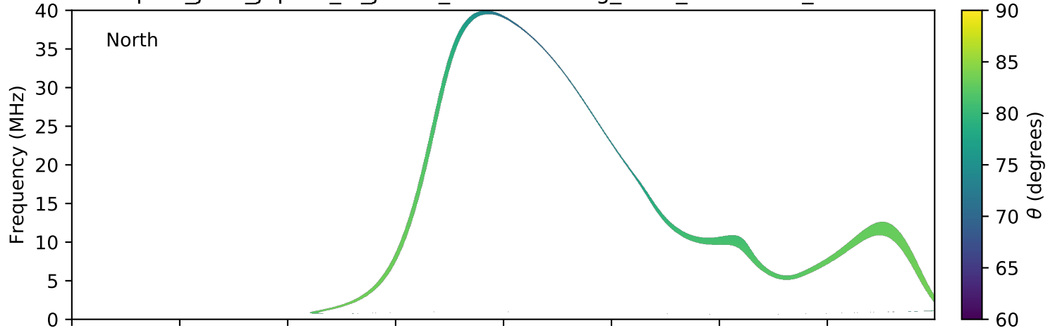
expres_juno_jupiter_io_jrm09_lossc-wid1deg_3kev_20180218_v01.cdf
