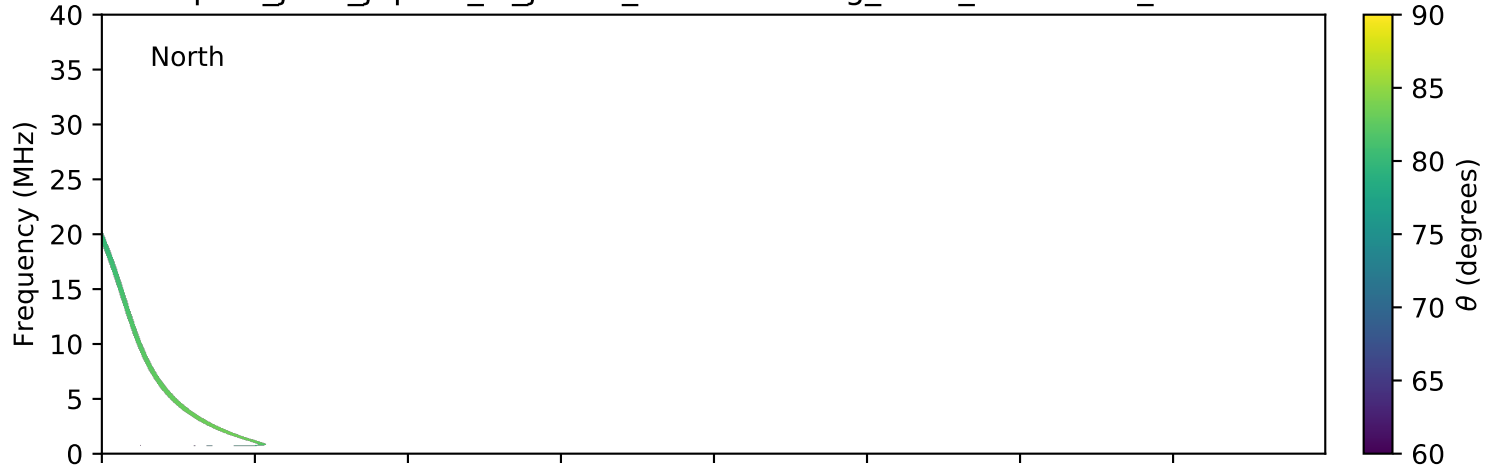
expres_juno_jupiter_io_jrm09_lossc-wid1deg_3kev_20180217_v01.cdf
