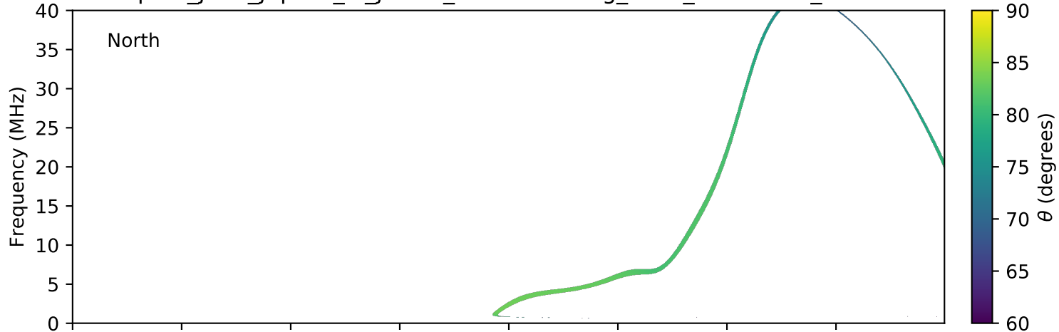
expres_juno_jupiter_io_jrm09_lossc-wid1deg_3kev_20180216_v01.cdf
