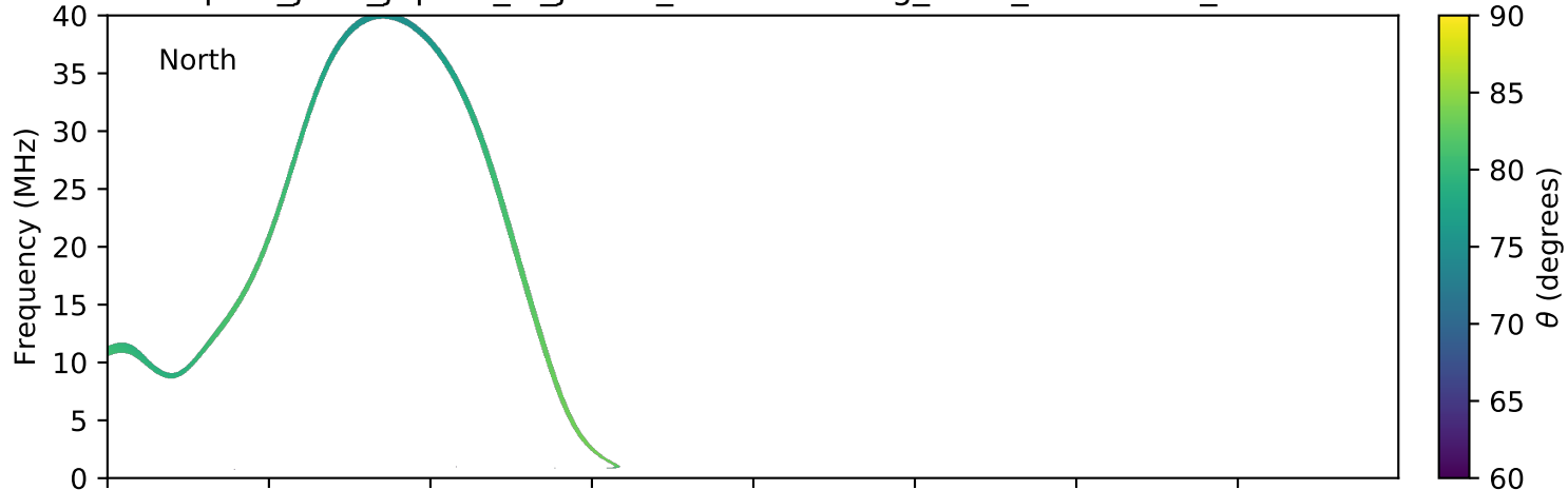
expres_juno_jupiter_io_jrm09_lossc-wid1deg_3kev_20180215_v01.cdf
