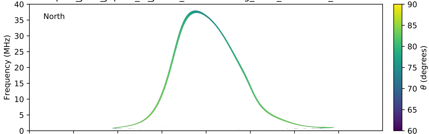
expres_juno_jupiter_io_jrm09_lossc-wid1deg_3kev_20180211_v01.cdf
