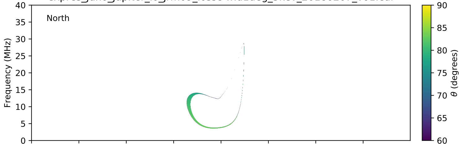
expres_juno_jupiter_io_jrm09_lossc-wid1deg_3kev_20180207_v01.cdf
