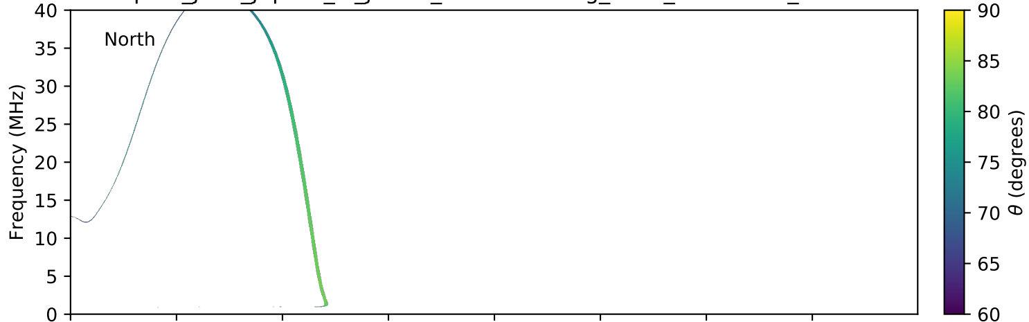
expres_juno_jupiter_io_jrm09_lossc-wid1deg_3kev_20180201_v01.cdf
