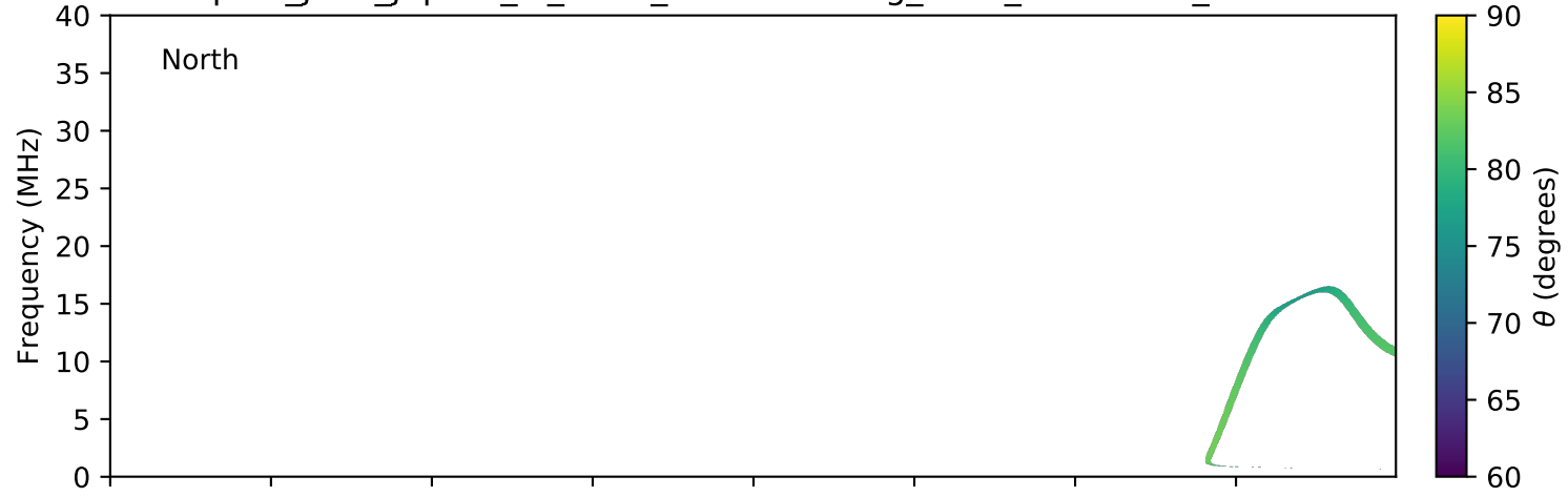
expres_juno_jupiter_io_isaac_lossc-wid1deg_3kev_20180228_v01.cdf
