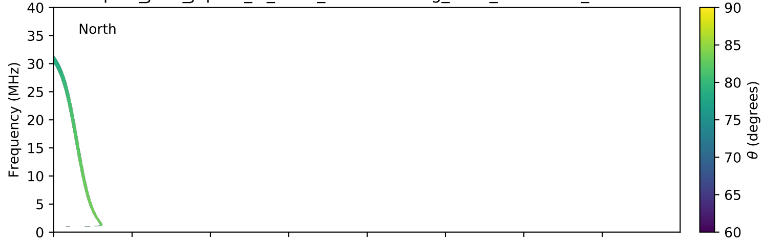
expres_juno_jupiter_io_isaac_lossc-wid1deg_3kev_20180226_v01.cdf
