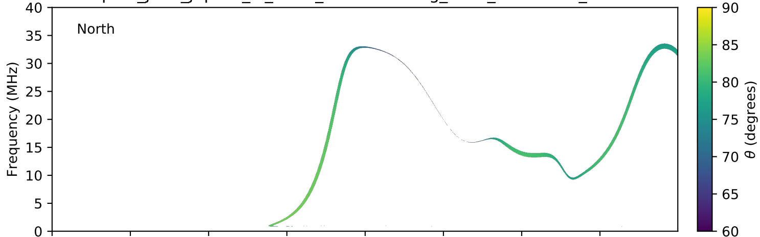
expres_juno_jupiter_io_isaac_lossc-wid1deg_3kev_20180225_v01.cdf
