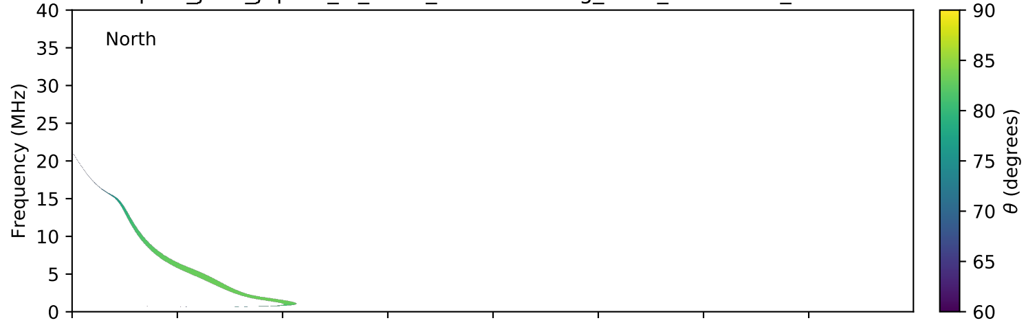
expres_juno_jupiter_io_isaac_lossc-wid1deg_3kev_20180224_v01.cdf
