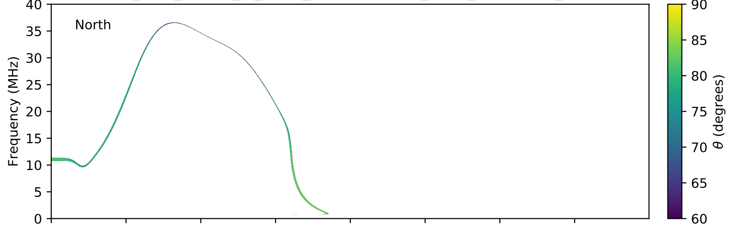
expres_juno_jupiter_io_isaac_lossc-wid1deg_3kev_20180222_v01.cdf
