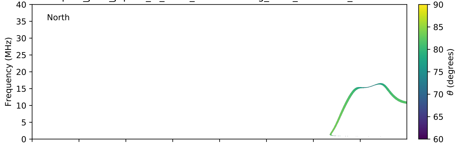
expres_juno_jupiter_io_isaac_lossc-wid1deg_3kev_20180221_v01.cdf
