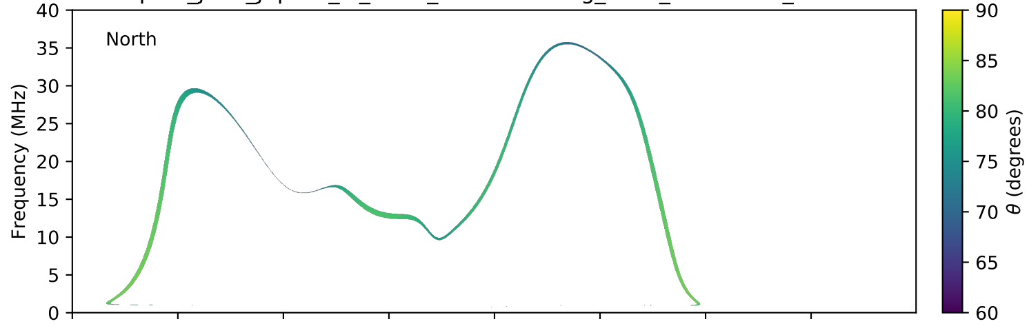
expres_juno_jupiter_io_isaac_lossc-wid1deg_3kev_20180220_v01.cdf
