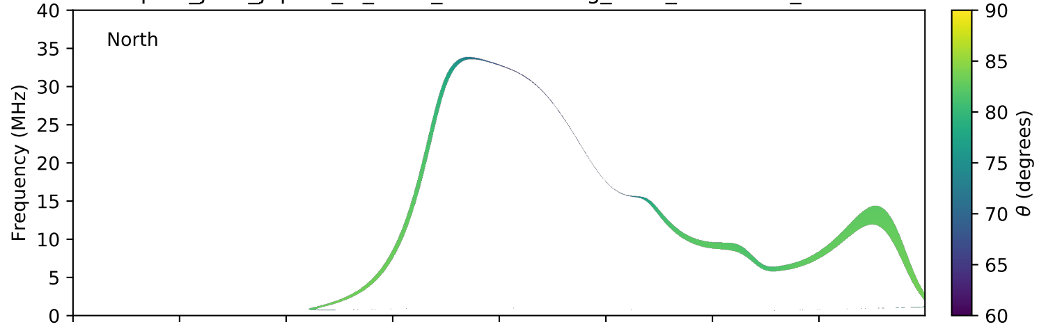
expres_juno_jupiter_io_isaac_lossc-wid1deg_3kev_20180218_v01.cdf
