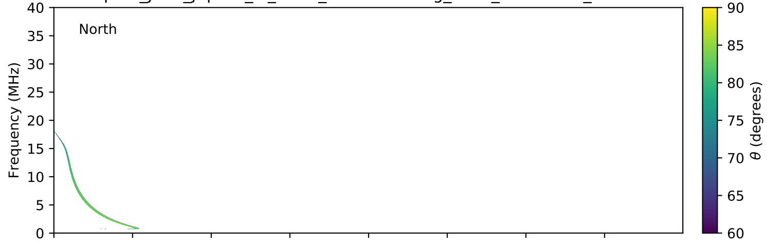
expres_juno_jupiter_io_isaac_lossc-wid1deg_3kev_20180217_v01.cdf
