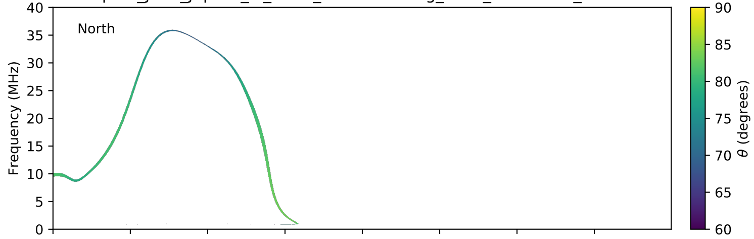
expres_juno_jupiter_io_isaac_lossc-wid1deg_3kev_20180215_v01.cdf
