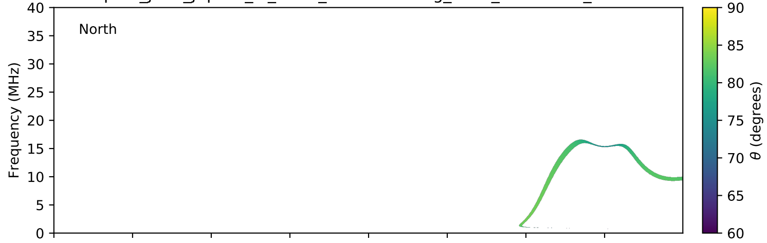
expres_juno_jupiter_io_isaac_lossc-wid1deg_3kev_20180214_v01.cdf
