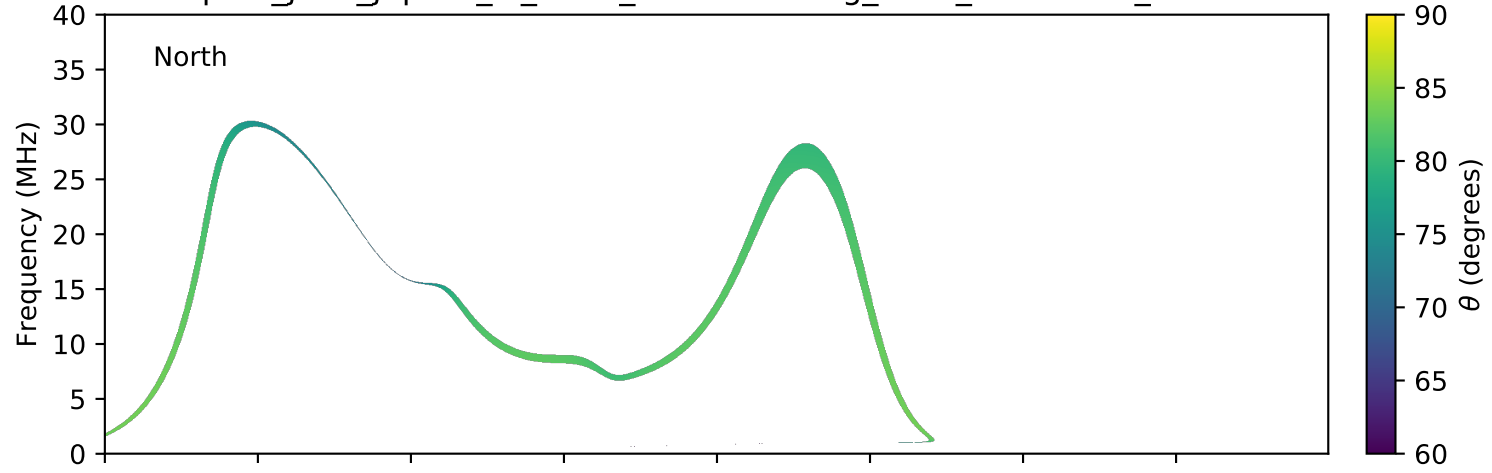
expres_juno_jupiter_io_isaac_lossc-wid1deg_3kev_20180213_v01.cdf
