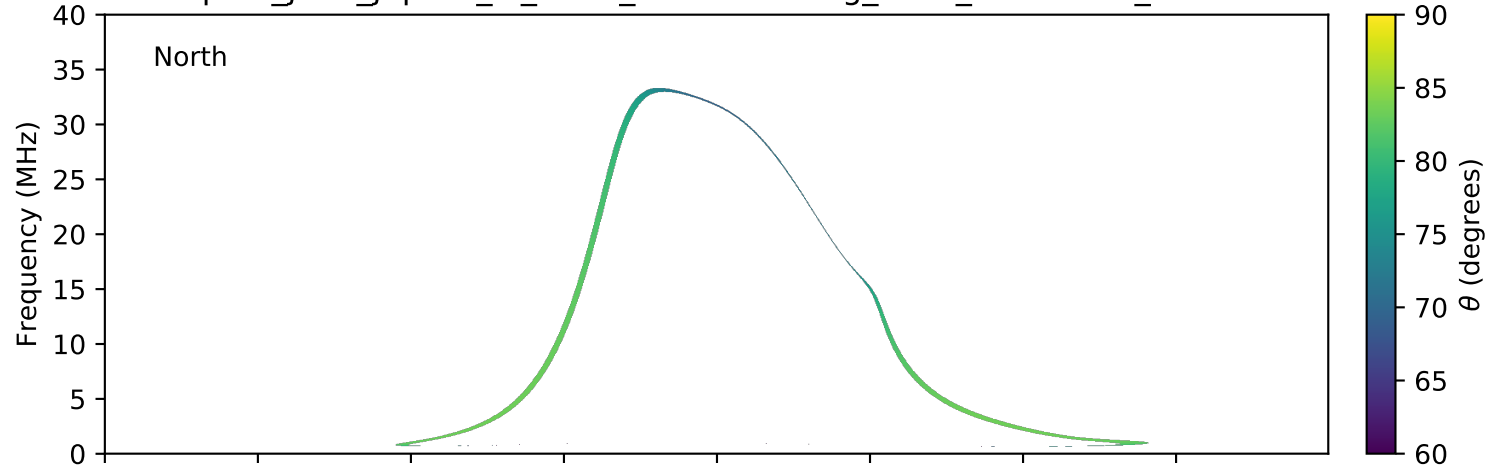
expres_juno_jupiter_io_isaac_lossc-wid1deg_3kev_20180211_v01.cdf
