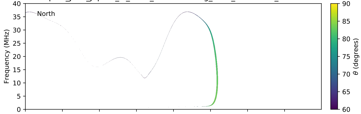
expres_juno_jupiter_io_isaac_lossc-wid1deg_3kev_20180206_v01.cdf
