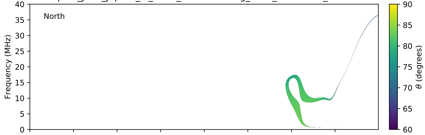
expres_juno_jupiter_io_isaac_lossc-wid1deg_3kev_20180205_v01.cdf
