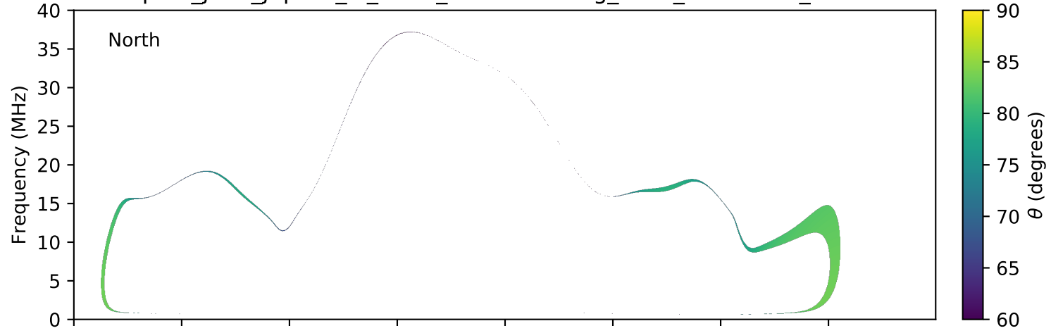
expres_juno_jupiter_io_isaac_lossc-wid1deg_3kev_20180204_v01.cdf
