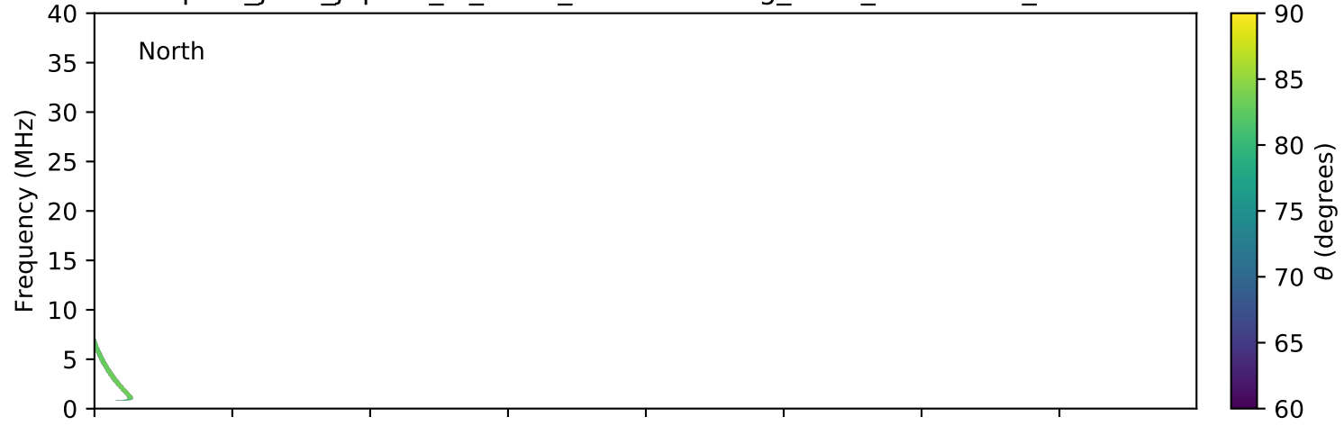
expres_juno_jupiter_io_isaac_lossc-wid1deg_3kev_20180203_v01.cdf
