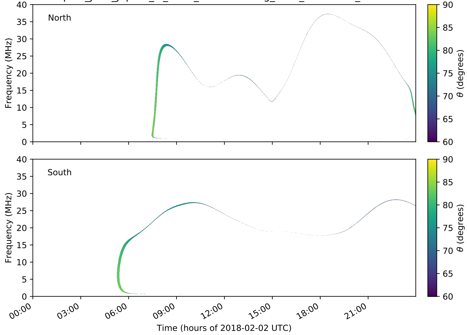
expres_juno_jupiter_io_isaac_lossc-wid1deg_3kev_20180202_v01.cdf
