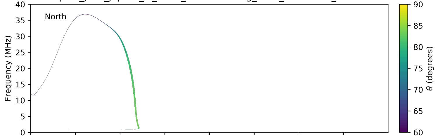
expres_juno_jupiter_io_isaac_lossc-wid1deg_3kev_20180201_v01.cdf
