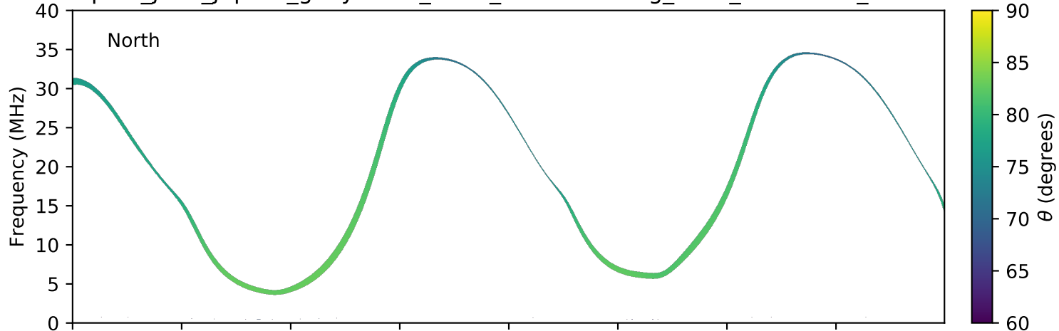
expres_juno_jupiter_ganymede_isaac_lossc-wid1deg_3kev_20180228_v01.cdf
