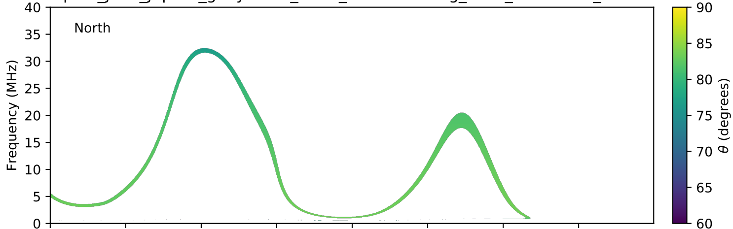
expres_juno_jupiter_ganymede_isaac_lossc-wid1deg_3kev_20180222_v01.cdf
