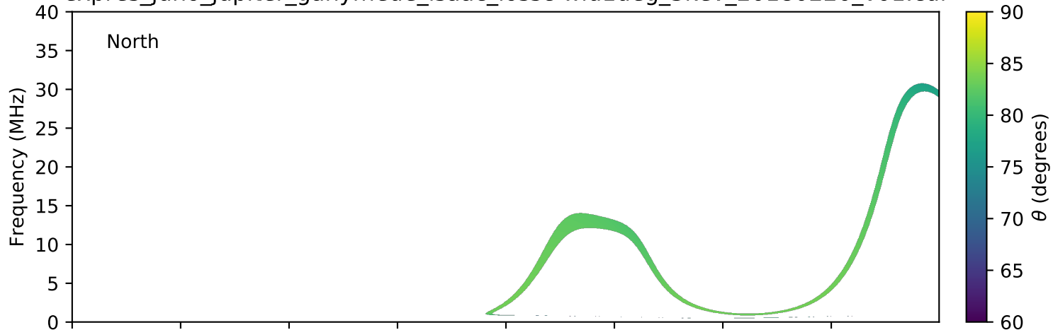
expres_juno_jupiter_ganymede_isaac_lossc-wid1deg_3kev_20180220_v01.cdf
