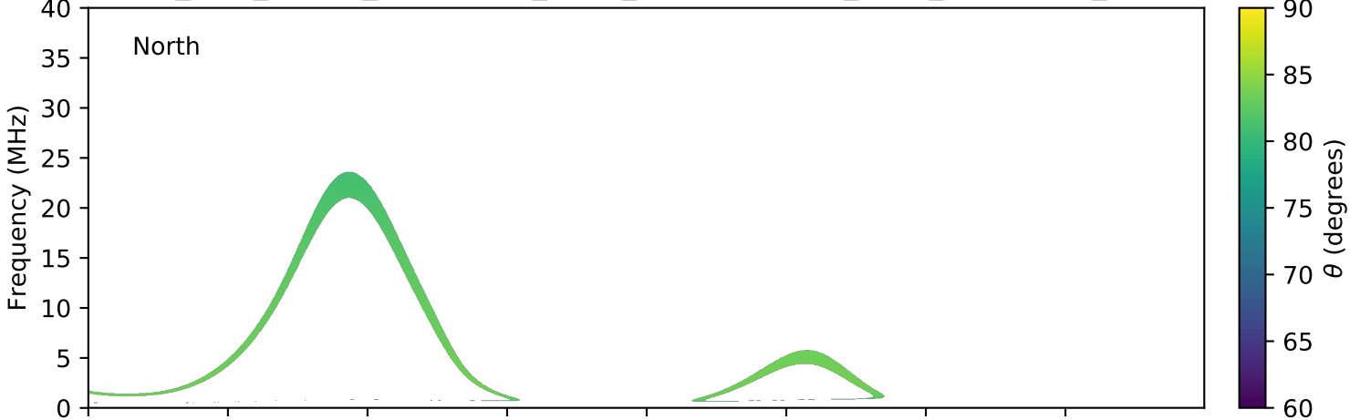
expres_juno_jupiter_ganymede_isaac_lossc-wid1deg_3kev_20180215_v01.cdf
