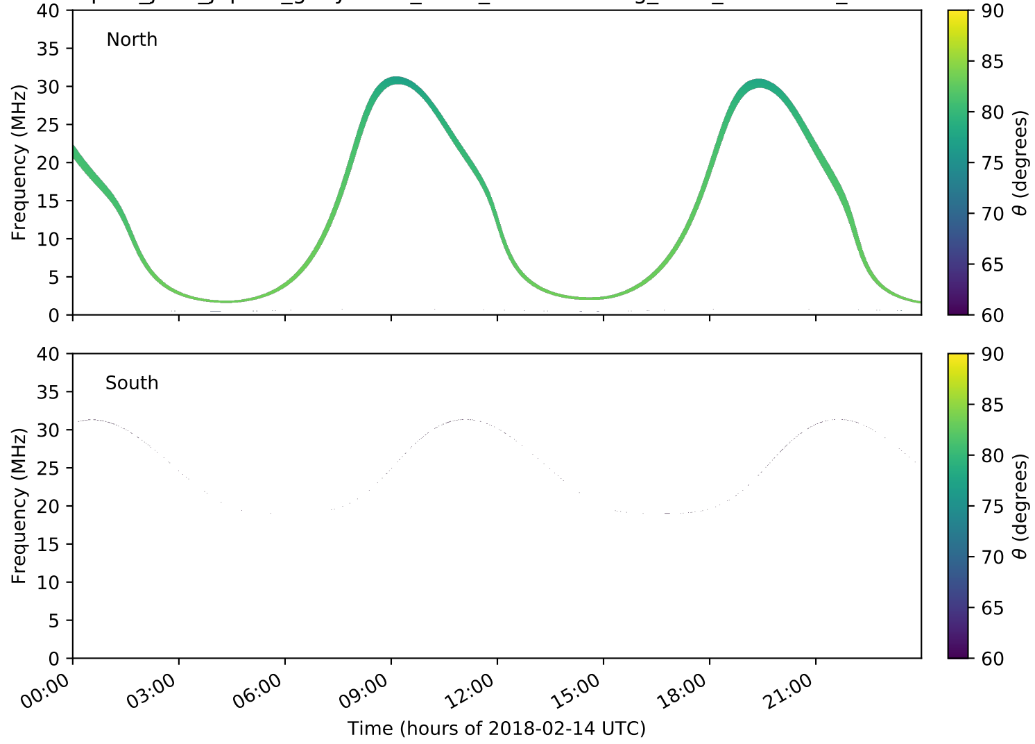
expres_juno_jupiter_ganymede_isaac_lossc-wid1deg_3kev_20180214_v01.cdf
