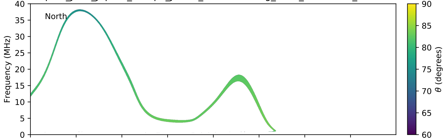
expres_juno_jupiter_europa_jrm09_lossc-wid1deg_3kev_20180225_v01.cdf
